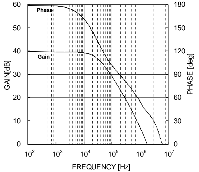
Figure 47. Voltage Gain • Phase – Frequency
