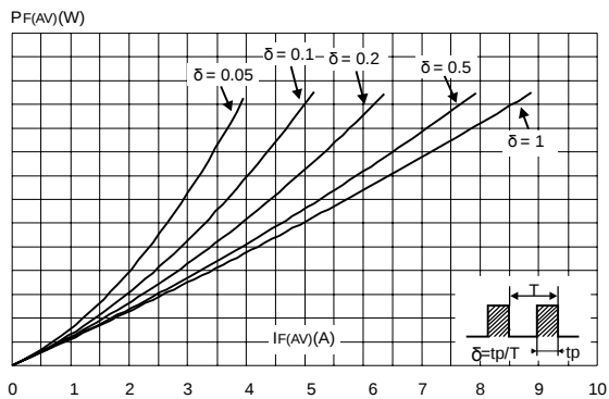
Figure 1: Conduction losses versus average current (per diode)
