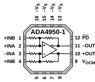
Figure 1. ADA4950-1
