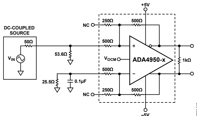
Figure 49. Equivalent Basic Test Circuit, G = 1
