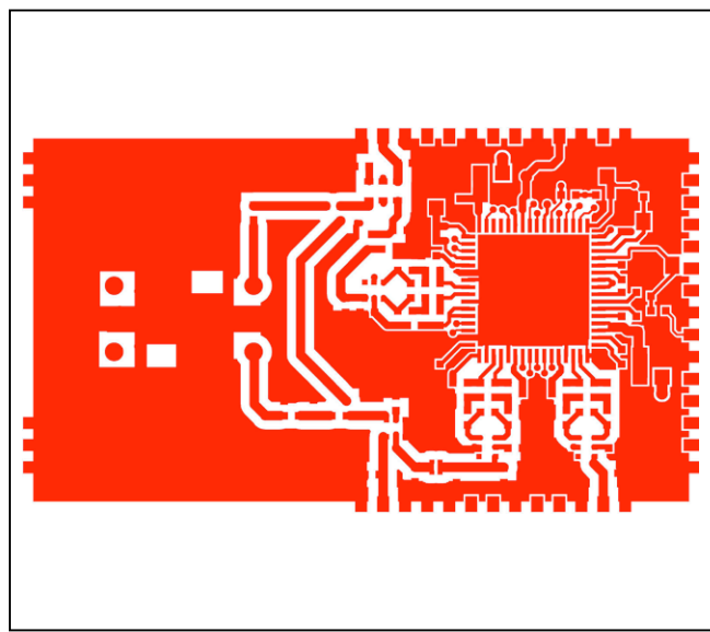
SC1905-DB2400—PCB Layout—Top
