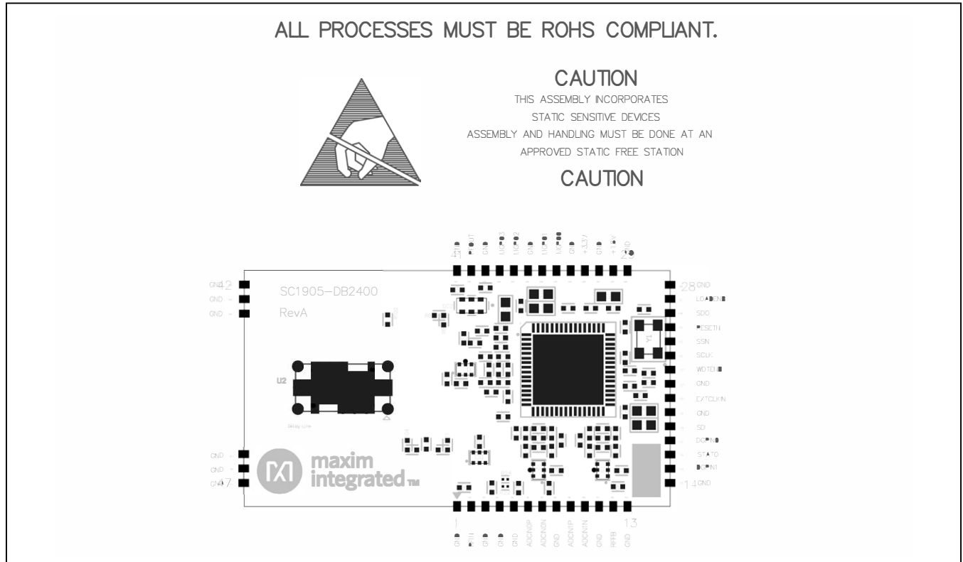
SC1905-DB2400—Assembly Drawing
