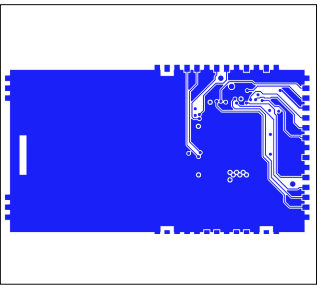
SC1905-DB2400—PCB Layout—Bottom
