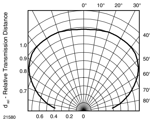
Fig. 13 - Vertical Directivity
