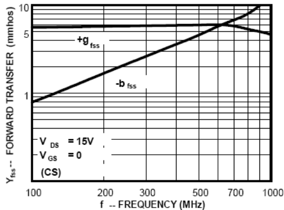
Forward Transadmittance
