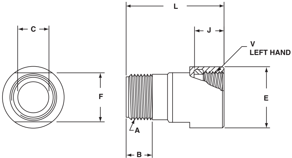
10-350695-XX( ) adapter
