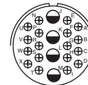
28-11 Service Rating: A Number of Contacts: 4 18 Contact Size: 12 16
