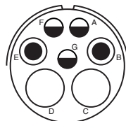
28-10 Service Rating: G = D; Bal. = A Number of Contacts: 2 2 3 Contact Size: 4 8 12
