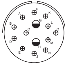
32-4 Service Rating F, J, K, N = A; Bal. = D Number of Contacts 2 12 Contact Size 12 16
