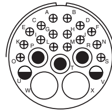
32-6 Service Rating A Number of Contacts 2 3 2 16 Contact Size 4 8 12 16
