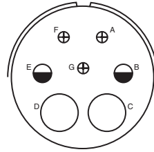
32-10 Service Rating A, F = E, G = B; B, E = D; C, D = A Number of Contacts 2 2 3 Contact Size 4 8 16
