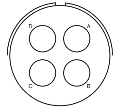
32-17 Service Rating D Number of Contacts 4 Contact Size 4
