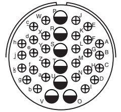
32-7 Service Rating A, B, h, j = Inst; Bal. = A Number of Contacts 7 28 Contact Size 12 16
