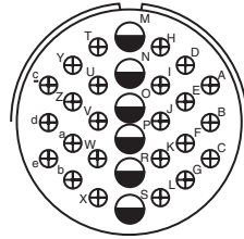
32-8 Service Rating A Number of Contacts 6 24 Contact Size 12 16
