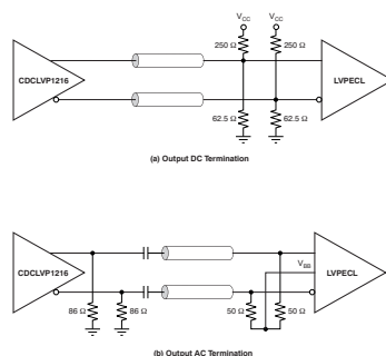
Figure 14. LVPECL Output DC and AC Termination for V_{CC} = 2.5\text{ V}
