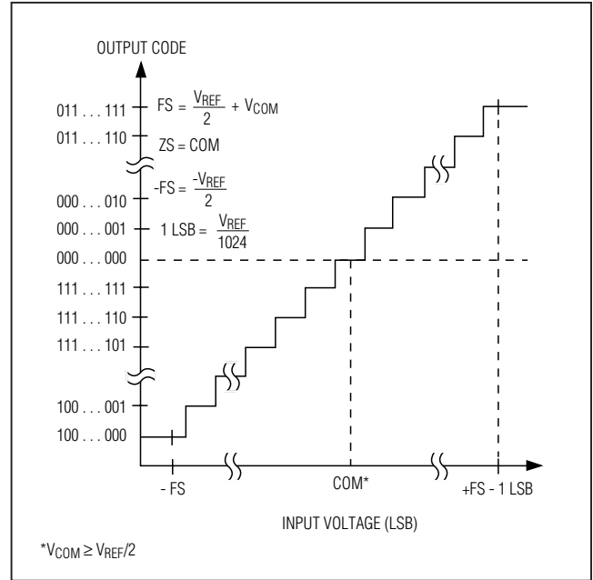
Figure 9. Bipolar Transfer Function, Full Scale (±FS) = ±VREF/2
