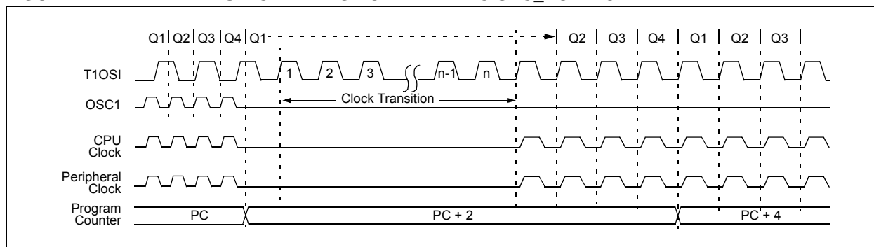
FIGURE 4-1: TRANSITION TIMING FOR ENTRY TO SEC RUN MODE
