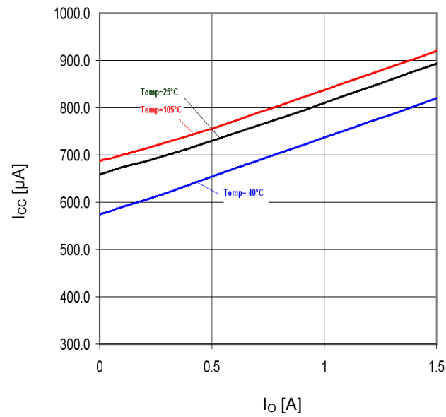
Figure 32. I_O - I_{CC}
