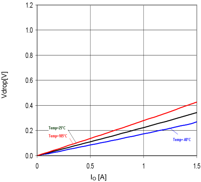
Figure 38. Minimum dropout Voltage 2 (V CC =12V, Ta=25°C)
