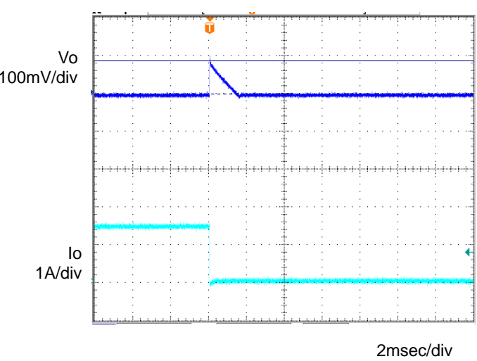
Figure 6. Transient Response (1.0→0A) Co=1μF, Ta=-40°C
