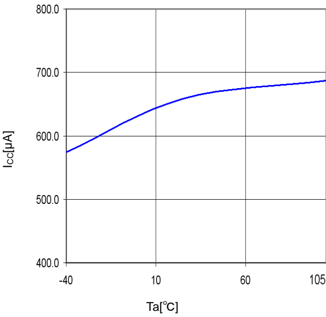
Figure 22. T_a - I_{CC}
