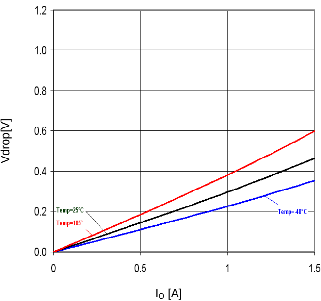
Figure 35. Minimum dropout Voltage 2 (V CC =6V, Ta=25°C)
