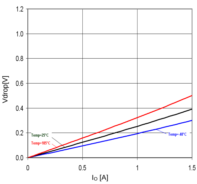
Figure 36. Minimum dropout Voltage 2 (V CC =8V, Ta=25°C)
