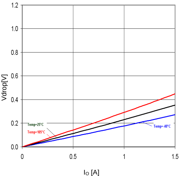
Figure 37. Minimum dropout Voltage 2 (V CC =10V, Ta=25°C)
