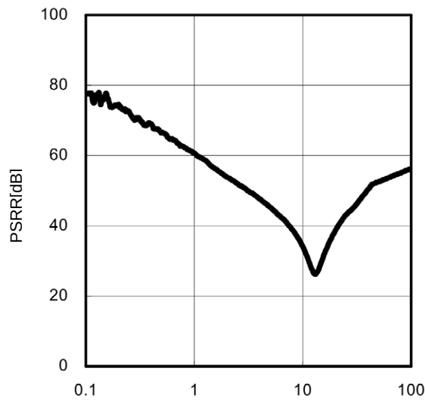
Figure 33. PSRR( I_O=0mA )
