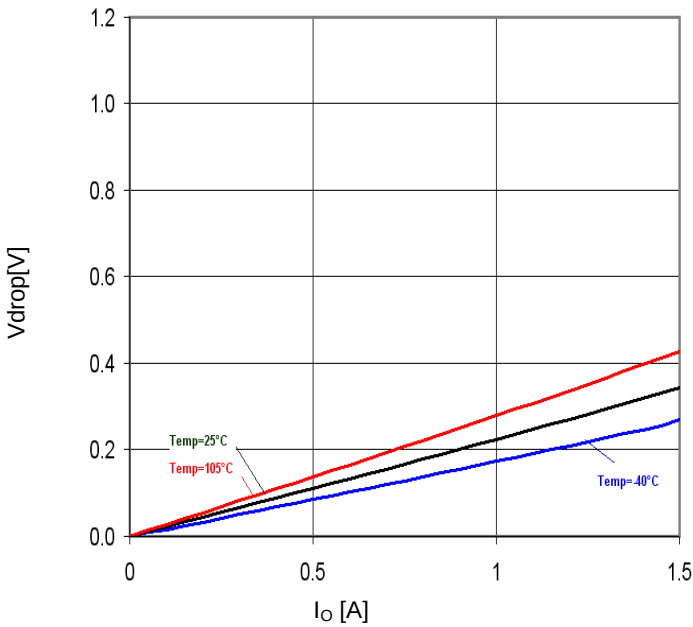
Figure 38. Minimum dropout Voltage 2 (V CC =12V, Ta=25°C)
