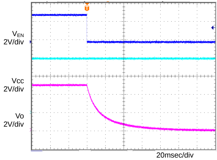
Figure 18. OFF sequence 2 C_o=1\mu F, T_a=-40^{\circ}C
