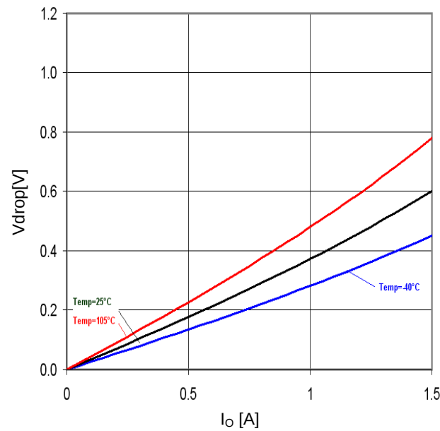
Figure 34. Minimum dropout Voltage 2 ( V_{CC} = 4.5 V, T_a = 25^\circ\text{C} )
