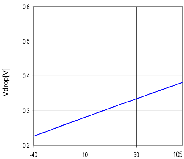
Figure 30. Minimum dropout Voltage1 ( V_{CC}=6\text{V} , I_O=1.0\text{A} )
