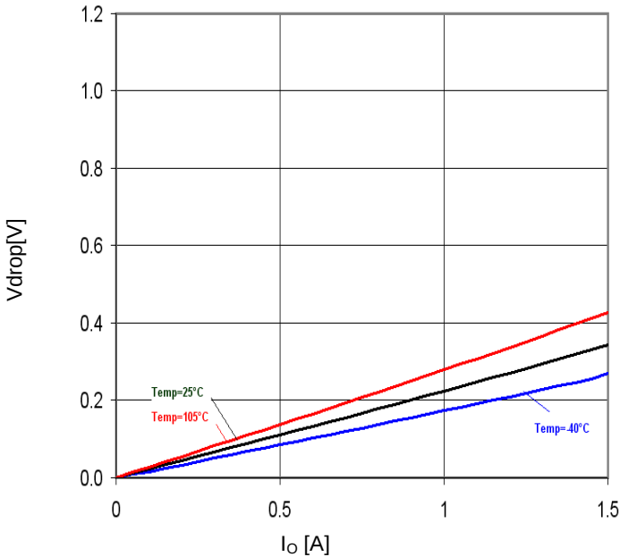
Figure 38. Minimum dropout Voltage 2 (V CC =12V, T a =25°C)
