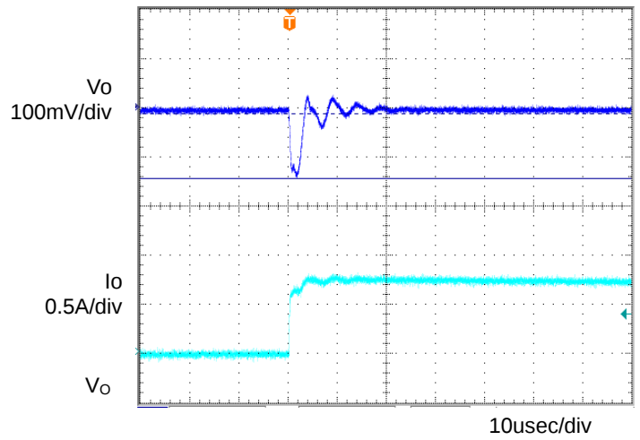
Figure 4. Transient Response (1.0→0A) C_o=1\mu F , T_a=25^\circ C
