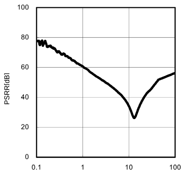
Figure 33. PSRR( I_O=0 mA)
