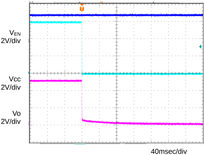
Figure 13. OFF sequence 1 C_o=1\mu F, T_a=25^{\circ}C
