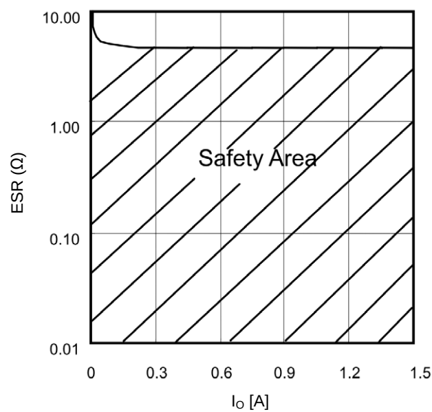
Figure 31. Operation Safety area
