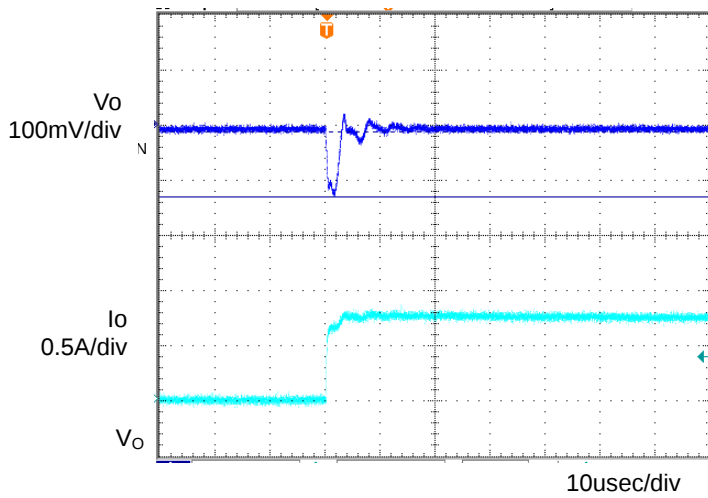
Figure 3. Transient Response (0→1.0A) C_o=1\mu F , T_a=-40^\circ C
