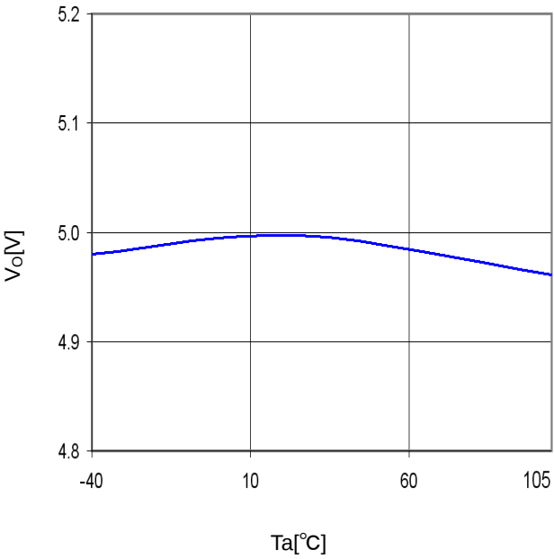
Figure 21. T_a - V_o ( I_o = 0\text{mA} )
