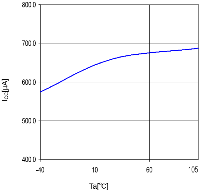
Figure 22. T_a - I_{cc}
