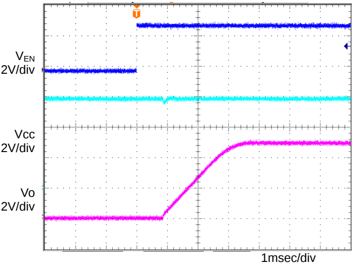
Figure 17. Input sequence 2 C_o=1\mu F, T_a=105^{\circ}C
