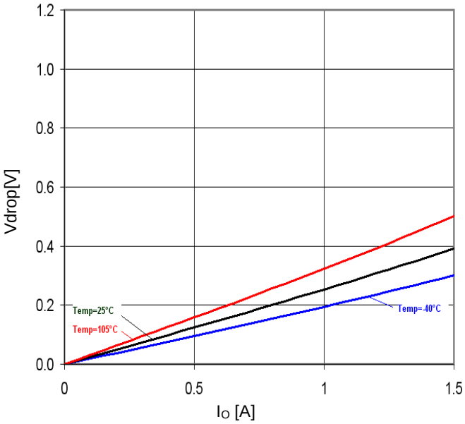
Figure 36. Minimum dropout Voltage 2 (V CC =8V, T a =25°C)
