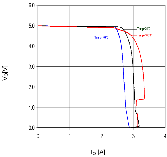
Figure 29. Io-Vo
