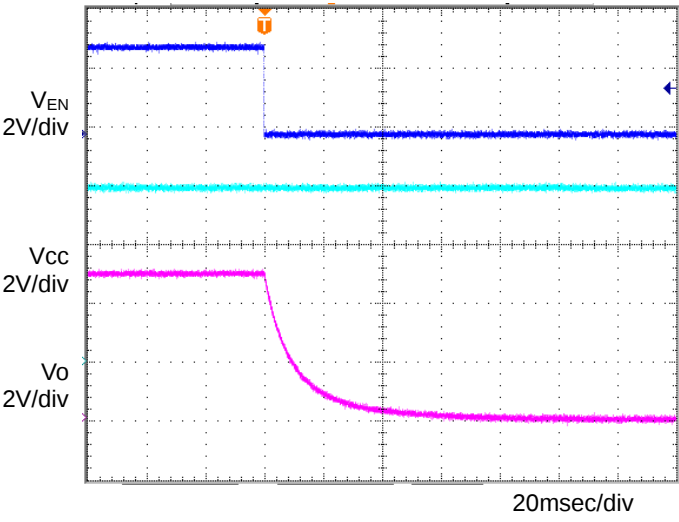
Figure 20. OFF sequence 2 C_o = 1\mu\text{F} , T_a = 105^\circ\text{C}
