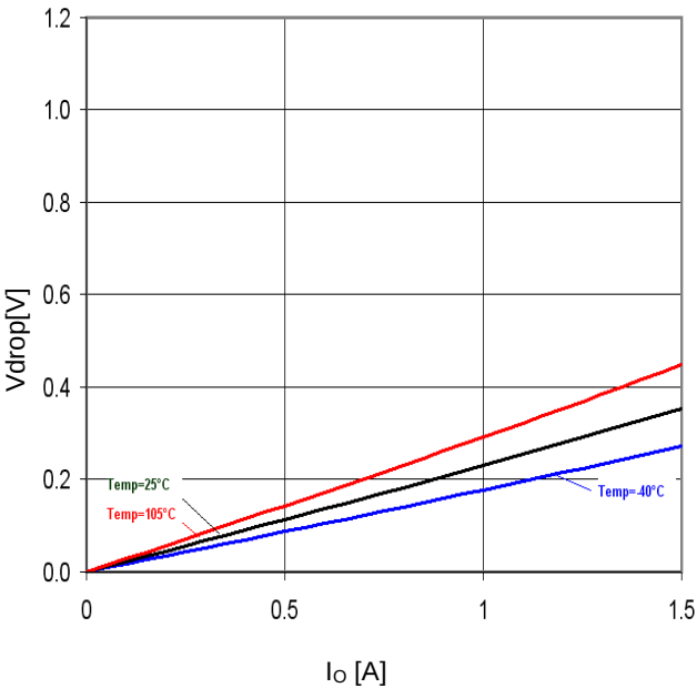
Figure 37. Minimum dropout Voltage 2 (V CC =10V, T a =25°C)
