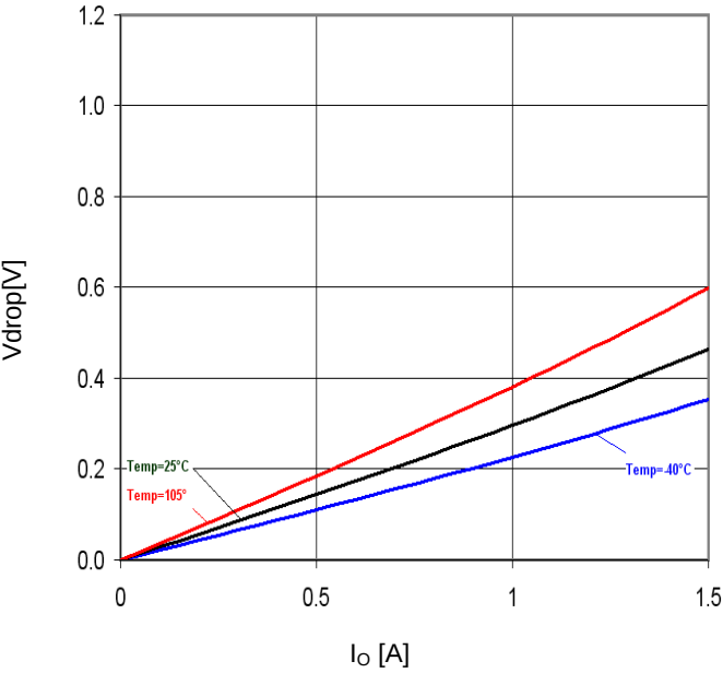
Figure 35. Minimum dropout Voltage 2 (V CC =6V, T a =25°C)
