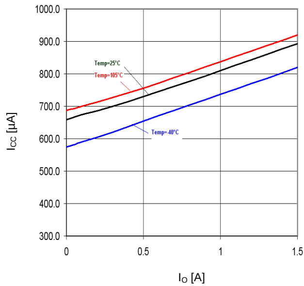
Figure 32. I_O - I_{CC}
