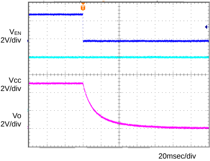
Figure 19. OFF sequence 2 C_o = 1\mu\text{F} , T_a = 25^\circ\text{C}
