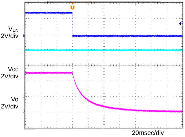
Figure 18. OFF sequence 2 C_o=1\mu F, T_a=-40^{\circ}C
