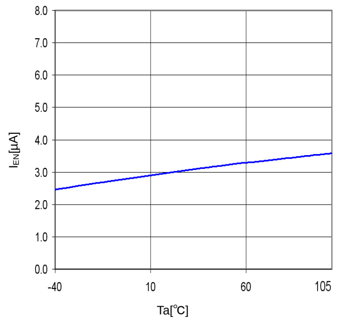
Figure 24. T_a - I_{EN}
