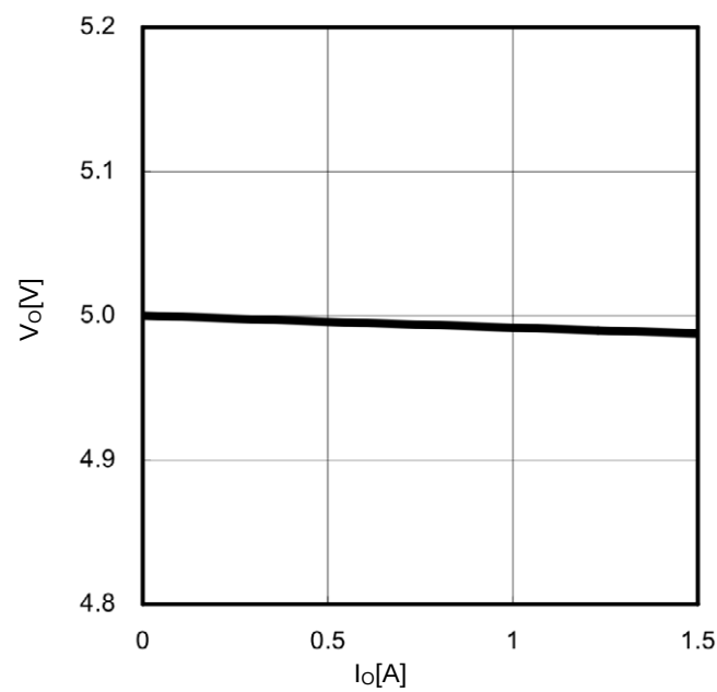
Figure.25. I_O - V_O
