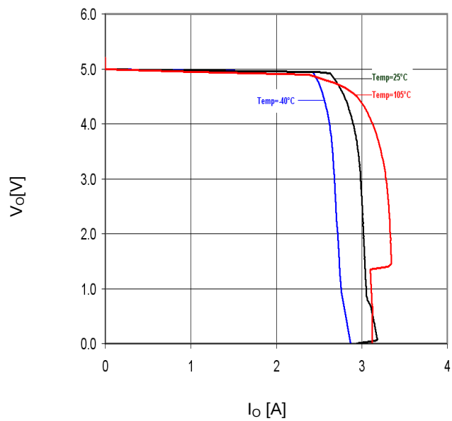
Figure 29. Io-Vo
