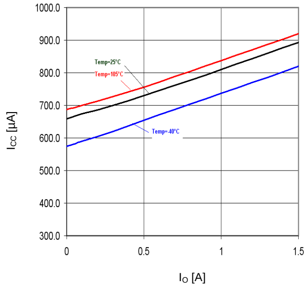
Figure 32. I_O - I_{CC}
