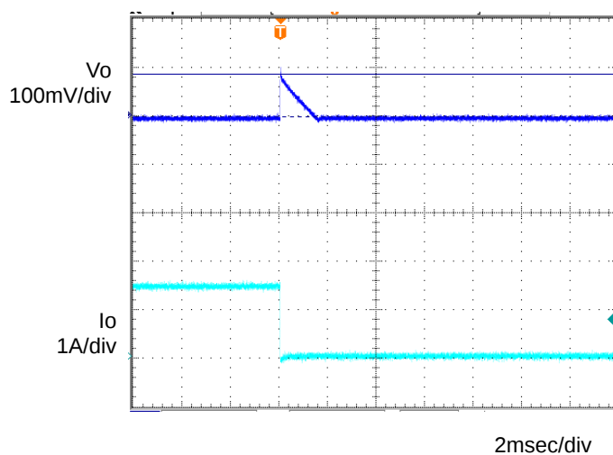
Figure 6. Transient Response (1.0→0A) C_o=1\mu F , T_a=-40^\circ C
