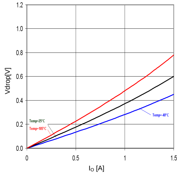
Figure 34. Minimum dropout Voltage 2 ( V_{CC}=4.5V , T_a=25^{\circ}C )
