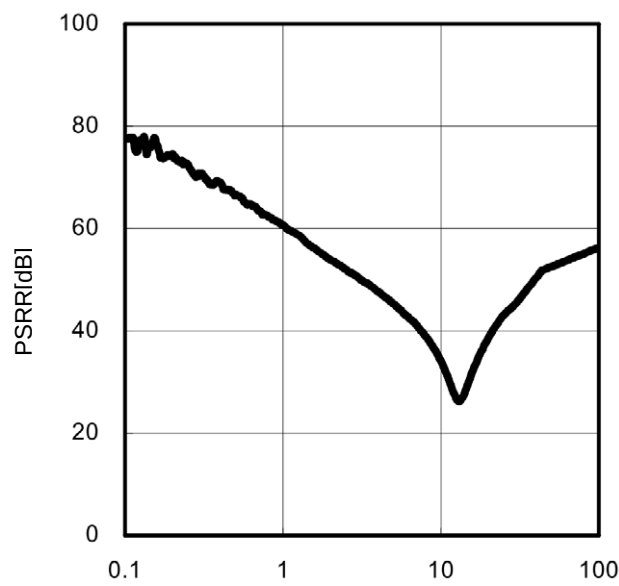
Figure 33. PSRR( I_O=0mA )
