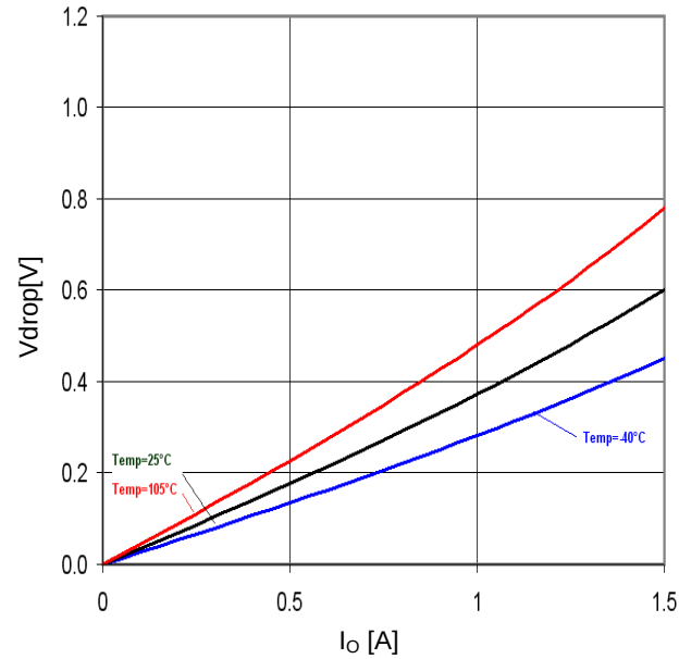
Figure 34. Minimum dropout Voltage 2 ( V_{CC}=4.5 V、 T_a=25^\circ\text{C} )
