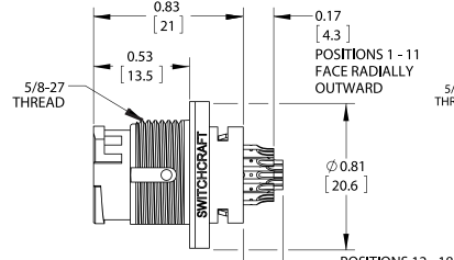
OPTION "C" EN3 SERIES 2-8 POSITION CRIMP TERMINALS EN3P2M26X SHOWN
