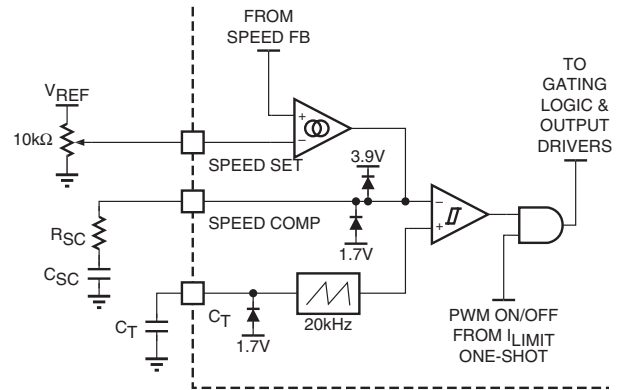
Figure 9. Speed Control Loop Component Connections
