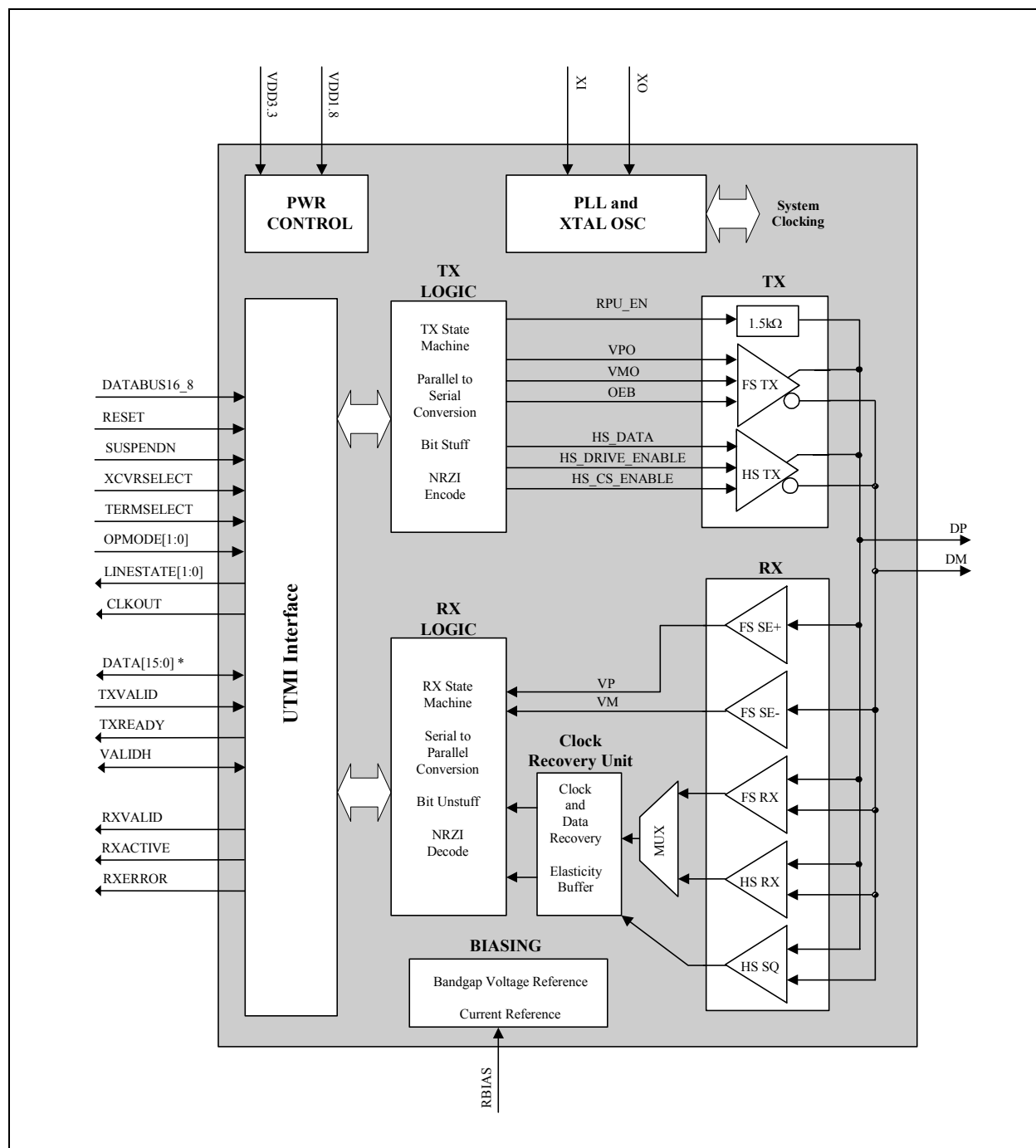
Figure 2.1 Block Diagram
