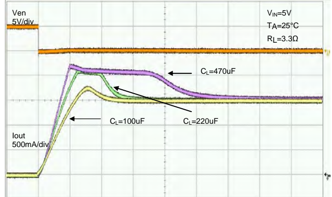
Inrush Current
