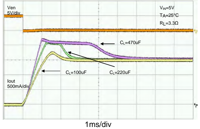
Inrush Current
