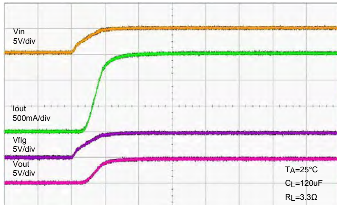
Power On with Full Load
