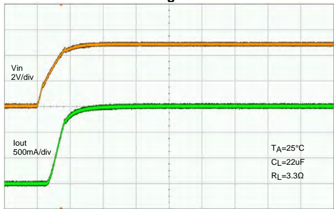
UVLO Increasing With Full Load
