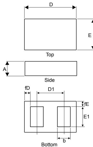
Figure 6. 0201 package outline
