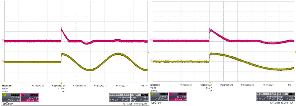
Figure 2: Inrush current, V_{in} = 115 \text{ VAC} , \text{Phase} = 90^\circ , CH1: V_{in} (200 V/div), CH2: I_{in} (10 A/div) Test data: the inrush current is 13 A at 115 VAC input
