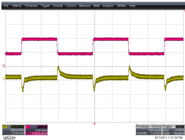
CH1: Vo (200 mV/div) CH2: I1 (5 A/div) Figure 15: Load transient VO, 5.25 A <-> 10.5 A (0.5 mS/div), 2 Aμs
