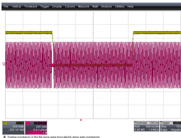
CH1:Vo (10 V/div) CH2:Vin (200 V/div) Figure 12: AC drop out 50 mS@230 VAC (50 mS/div), Vo restart
