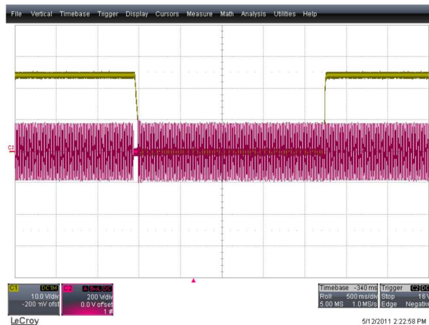
CH1:Vo (10 V/div) CH2:Vin (200 V/div) Figure 11: AC drop out 50 mS@115 VAC (50 mS/div), Vo restart
