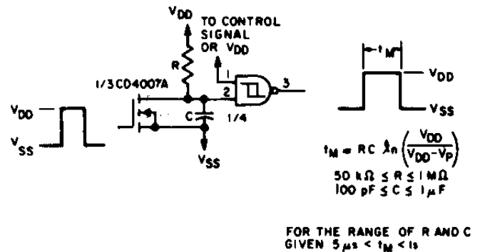
Figure 16. Monostable Multivibrator
