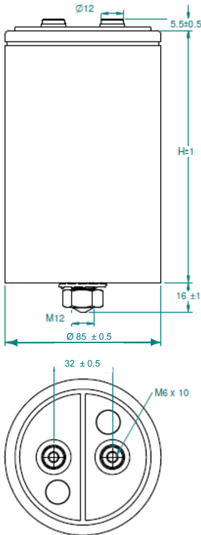
Figure 1: - B25620B - Ø 85mm - Female terminals (M6) - Between terminals 32±0.5mm
