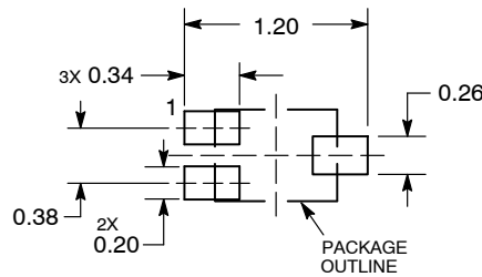
DIMENSIONS: MILLIMETERS
