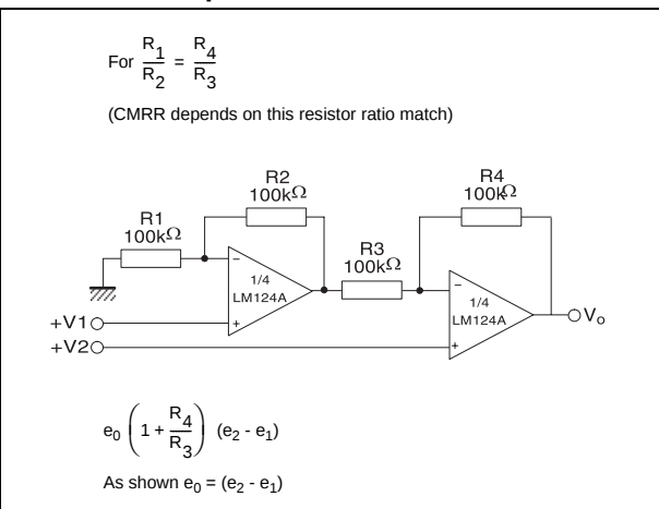
Figure 27. High input Z, DC differential amplifier
