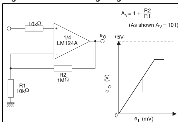
Figure 24. Non-inverting DC gain
