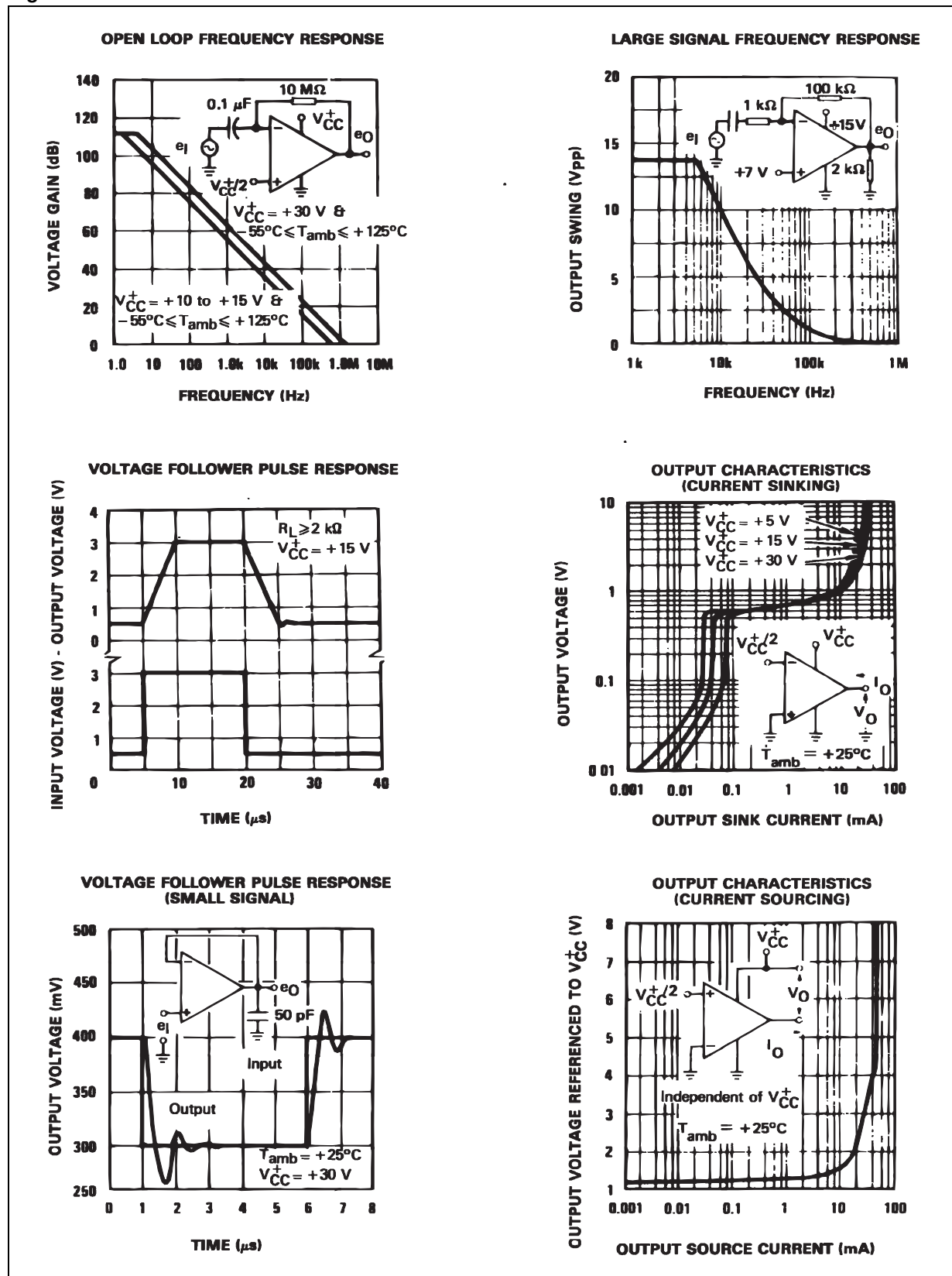
Figure 15. Electrical curves
