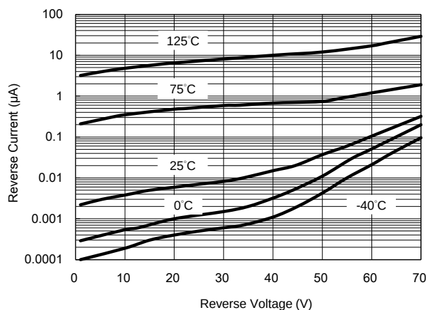
Fig. 2 Reverse Characteristics
