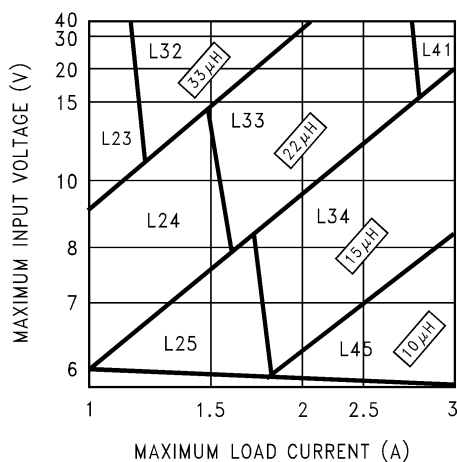
Figure 21. LM2670-3.3
