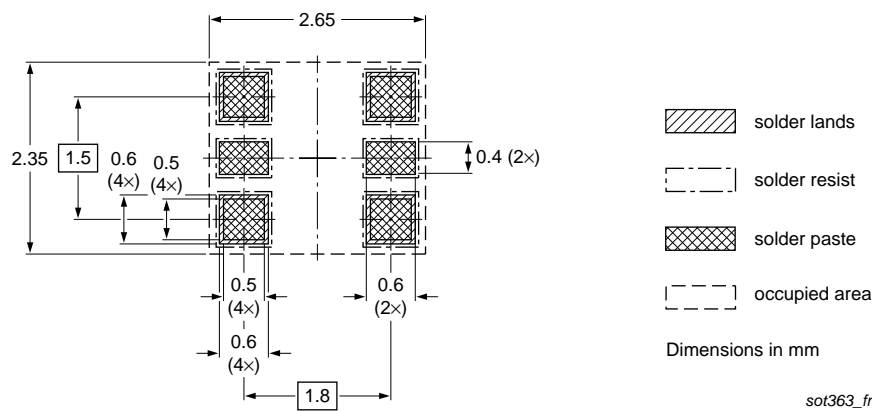
Fig 13. Reflow soldering footprint PUMH10 (SOT363/SC-88)
