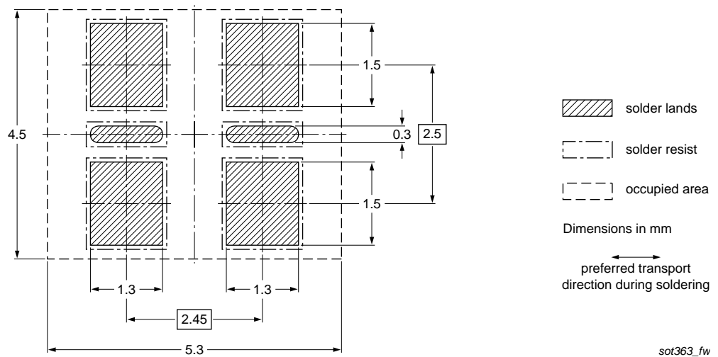
Fig 14. Wave soldering footprint PUMH10 (SOT363/SC-88)
