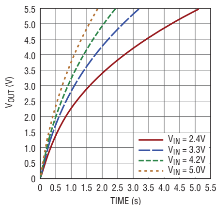
V_{OUT} vs Charge Time, C_{OUT} = 1F , R_{ESR} = 20m\Omega , I_{IN} = 2.0A
