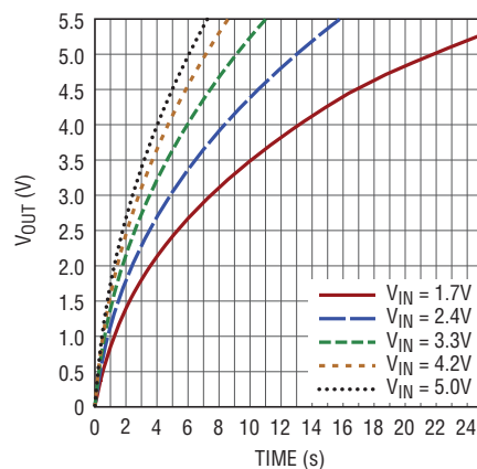
V_{OUT} vs Charge Time, C_{OUT} = 1F , R_{ESR} = 20m\Omega , I_{IN} = 0.5A
