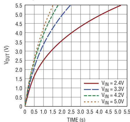
V_{OUT} vs Charge Time, C_{OUT} = 1F , R_{ESR} = 20m\Omega , I_{IN} = 3.0A
