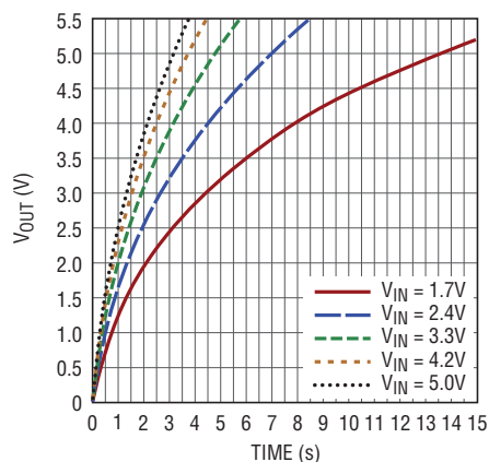
V_{OUT} vs Charge Time, C_{OUT} = 1F , R_{ESR} = 20m\Omega , I_{IN} = 1.0A
