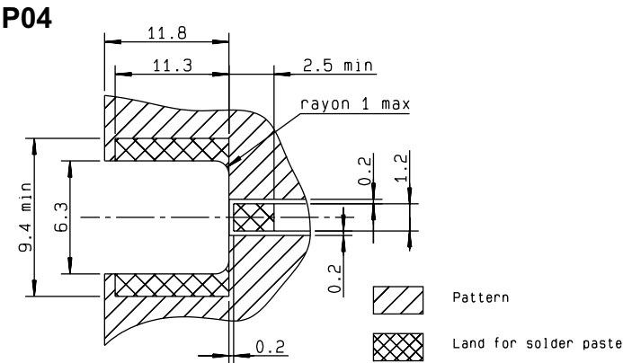
Receptacle soldering pattern PCB thickness : 1.6 mm
