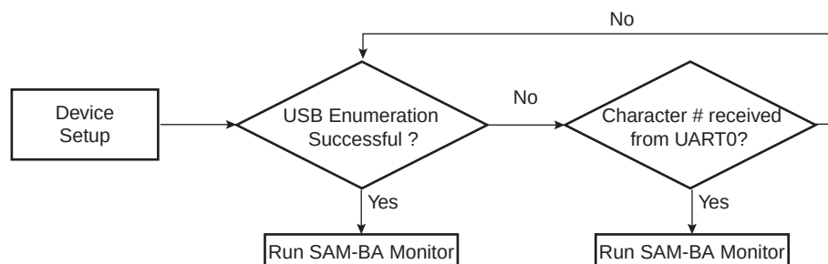
Figure 24-1. Boot Program Algorithm Flow Diagram
