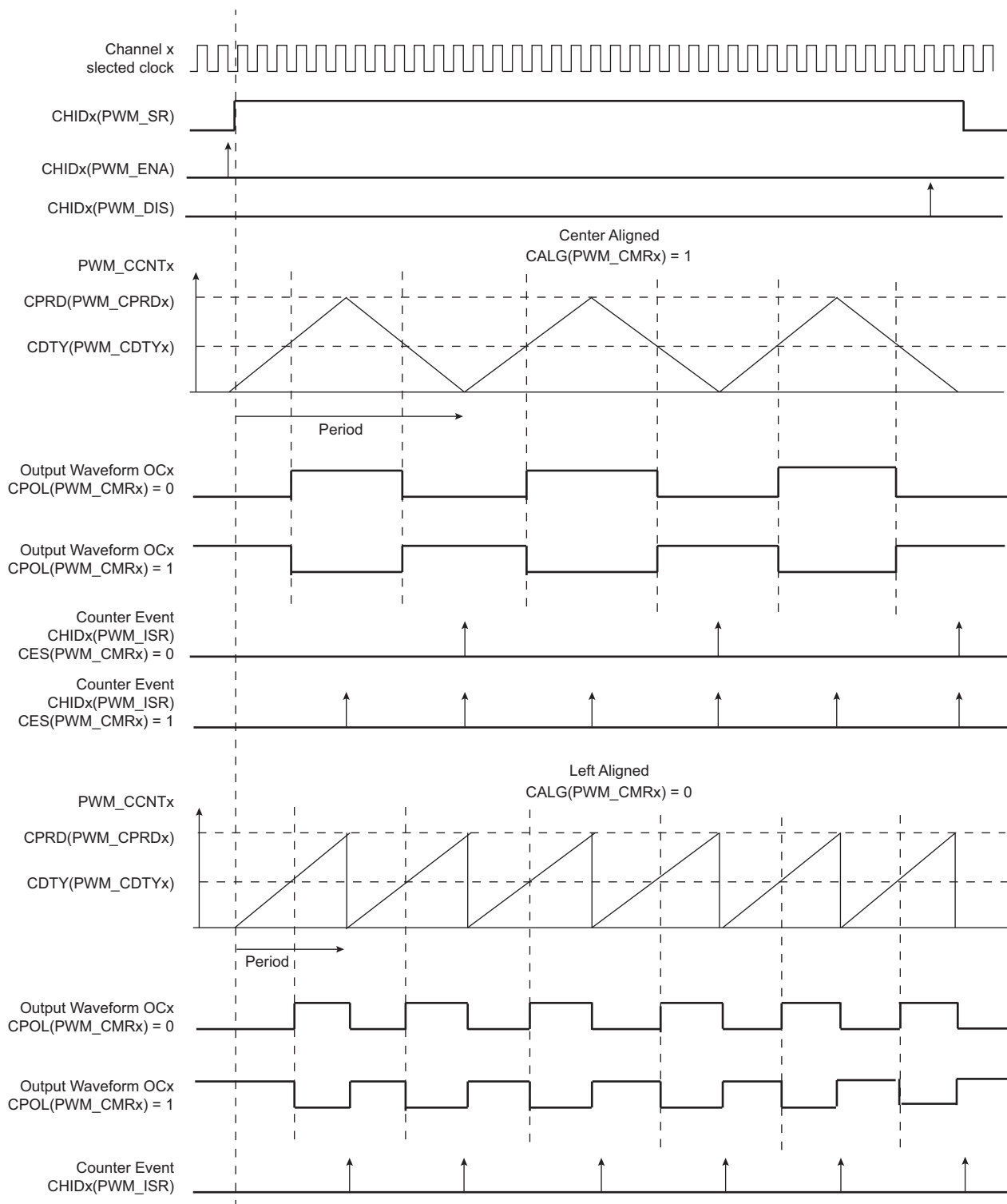
Figure 39-5. Waveform Properties
