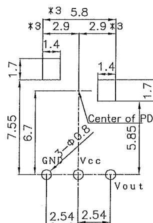
Example of mounting drawing from solder side (Reference)
