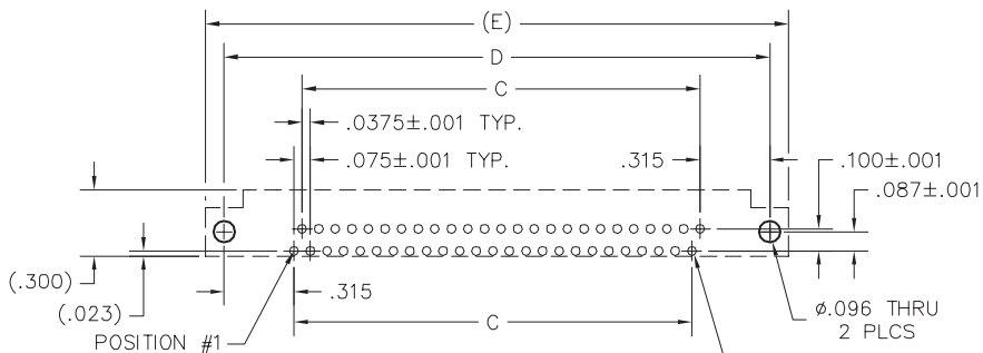
PCB LAYOUT VIEWED FROM COMPONENT SIDE
