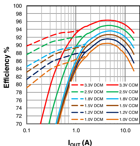
Figure 19: Efficiency, V_{IN}=5V
