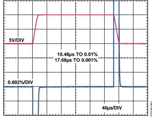
Figure 48. Large-Signal Pulse Response and Settling Time, G = 10, 10\text{ V Step}, V_S = \pm 15\text{ V}
