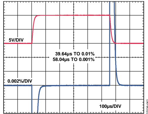
Figure 49. Large-Signal Pulse Response and Settling Time, G = 100, 10\text{ V Step}, V_S = \pm 15\text{ V}
