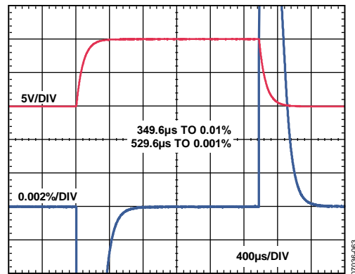
Figure 50. Large-Signal Pulse Response and Settling Time, G = 1000, 10\text{ V Step}, V_S = \pm 15\text{ V}
