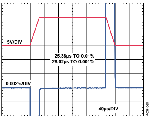
Figure 47. Large-Signal Pulse Response and Settling Time, G = 1, 10\text{ V Step}, V_S = \pm 15\text{ V}
