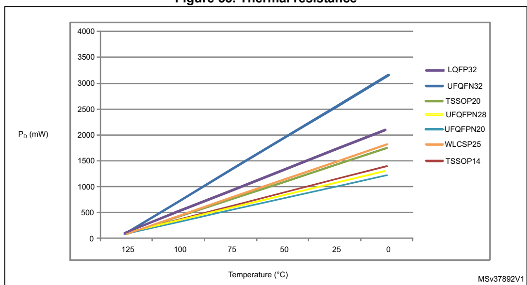
Figure 53. Thermal resistance
