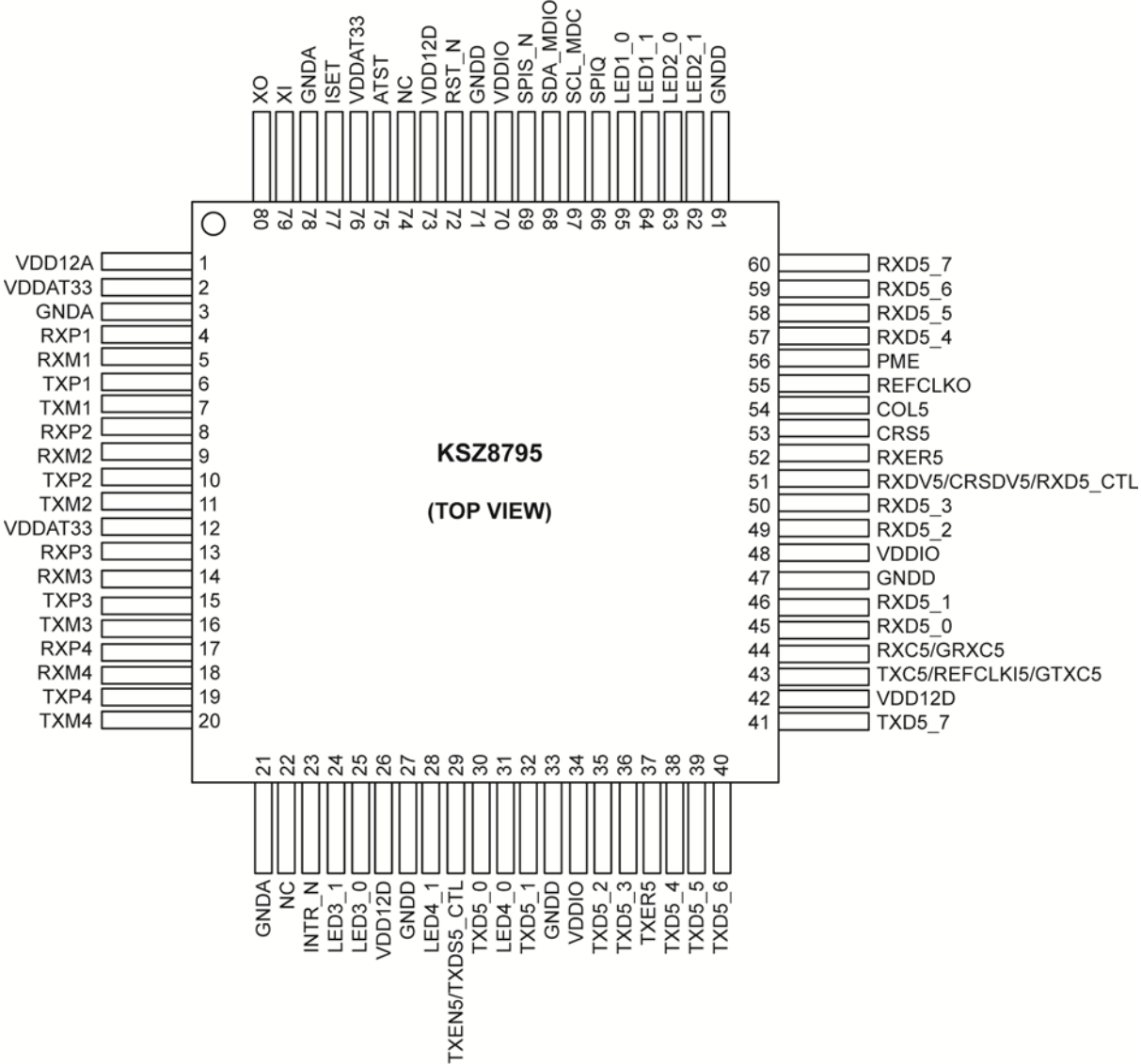
Figure 2. 80-Pin LQFP
