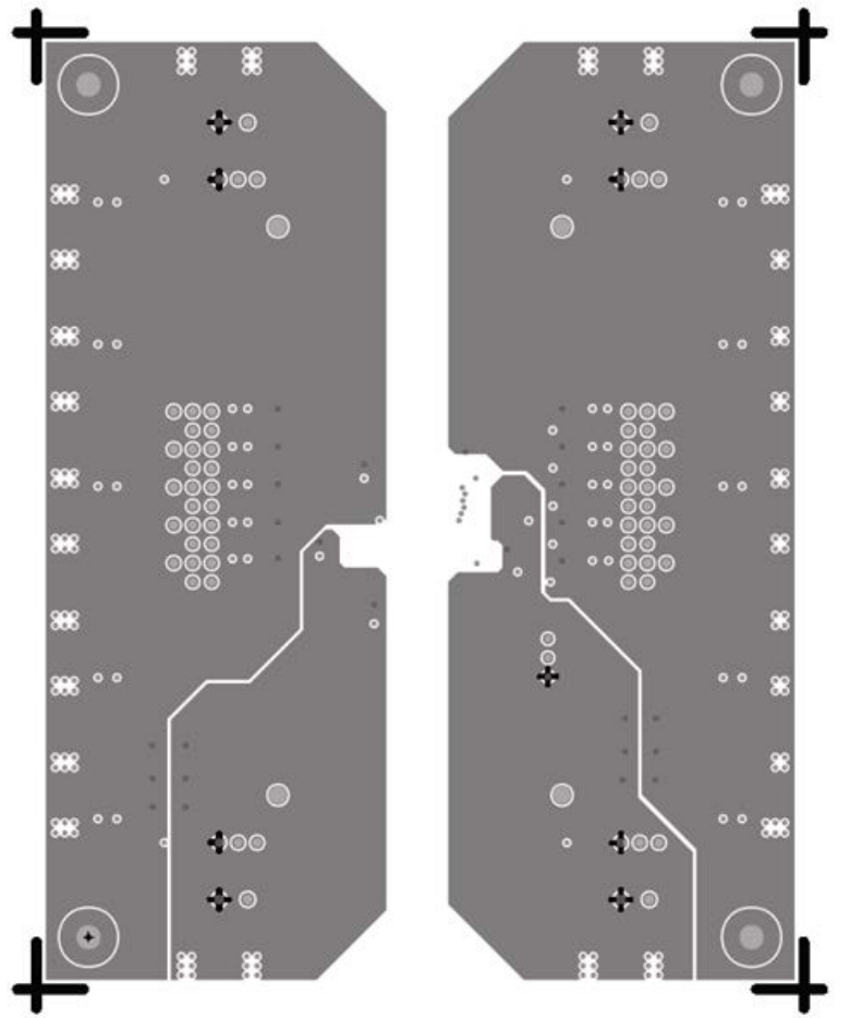
Figure 6. VDD1/VDDP/VDD2/VISO Power Planes (Layer 2)
