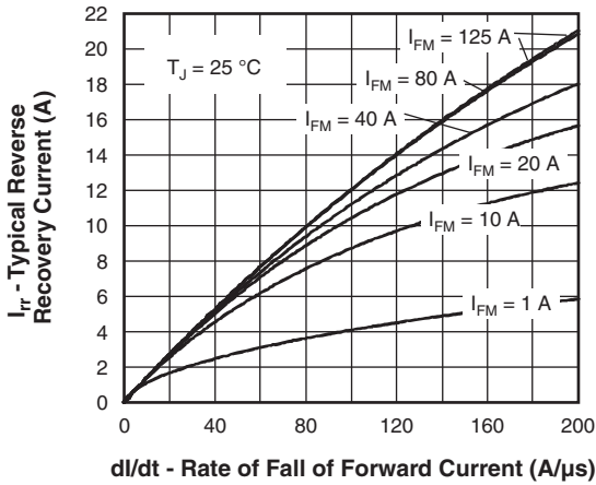
Fig. 12 - Recovery Current Characteristics, T_J = 25^\circ\text{C}
