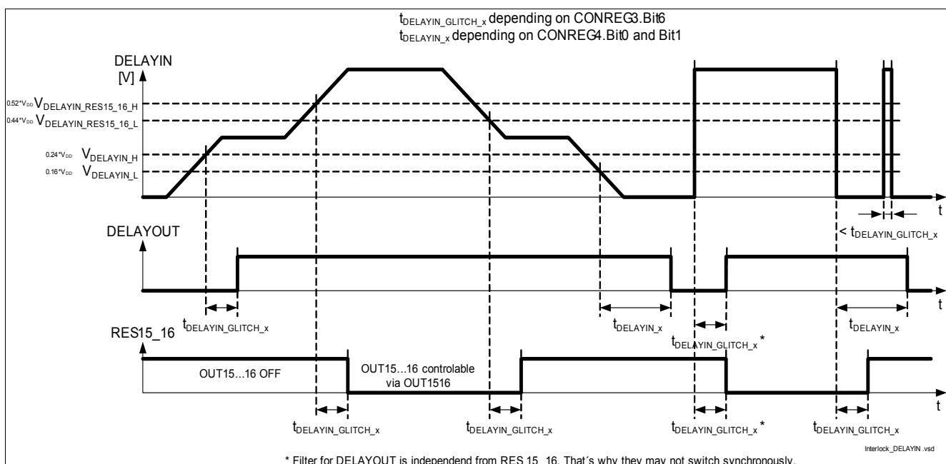
Figure 8 Timing DELAYIN
