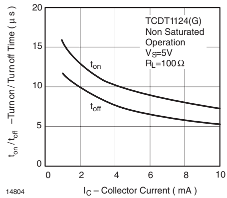
Figure 19. Turn on / off Time vs. Collector Current
