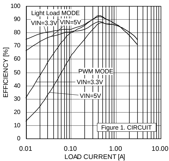
Figure 8. Efficiency(BD90525EFJ-C)
