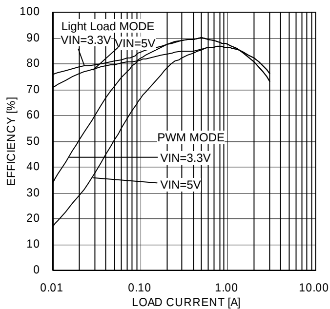
Figure 9. Efficiency(BD90528EFJ-C)
