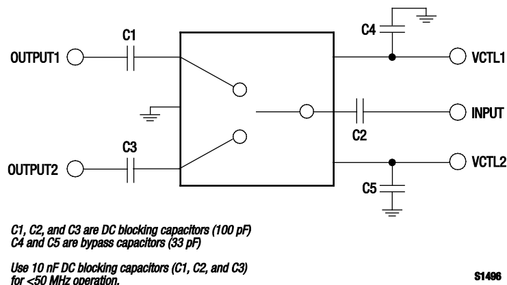
Figure 10. SKY13351-378LF Evaluation Board Schematic
