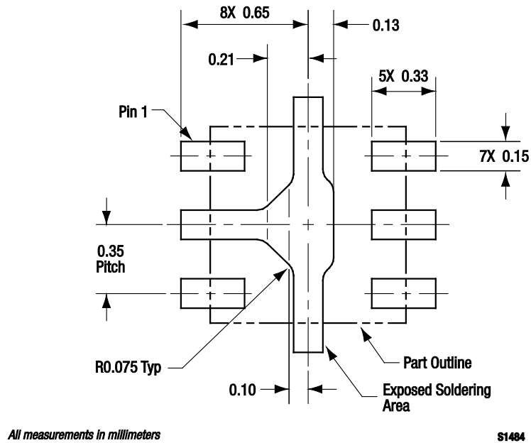
Figure 12. SKY13351-378LF PCB Layout Footprint (Top View)
