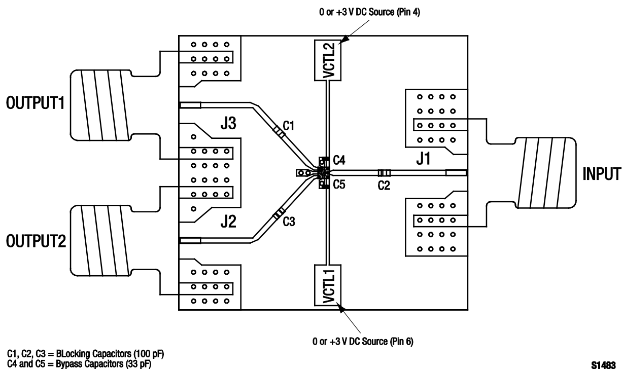
Figure 11. SKY13351-378LF Evaluation Board Assembly Diagram
